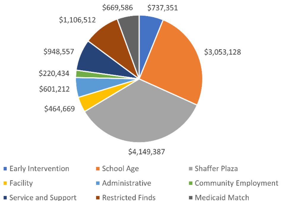
2023 Operating Costs
